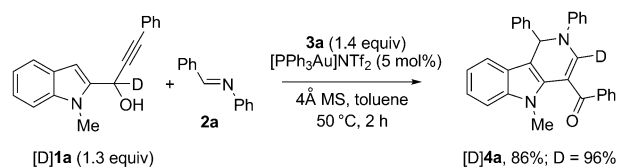
Scheme 6. Deuterium-labeling experiment.
